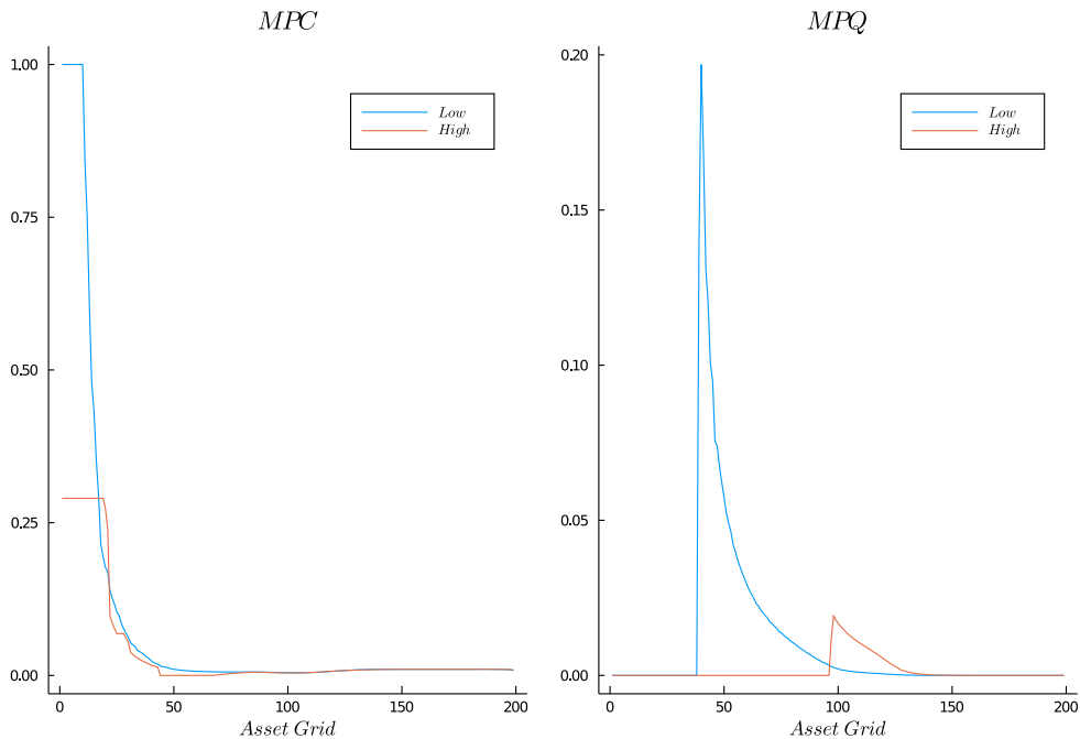
Figure 3: MPC and MPQ
